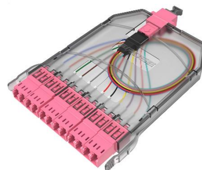
OC12 cassette For 144F/1U (12F*12pcs)
